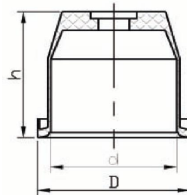
D - Clopot Ø 10.5 x Ø 51.5 x 40.5 cod - CL 1
